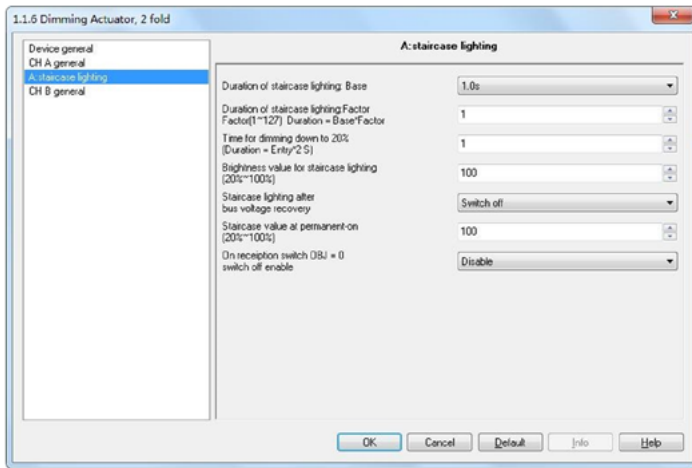
Fig. 6.7 parameter window "CH X staircase lighting"
